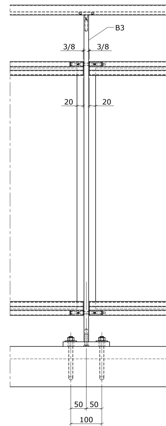
DETAIL B
